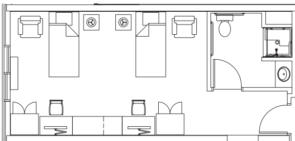
Floor Plan I
